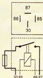
Mini Relay Make and Break, 12 volt, 15 amps, fitted with fuse.
