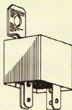
Mini Relay Normally Closed, circuit opens when energised, 12 volt, 20 amps.
