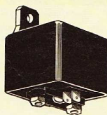
Heavy Duty Relay Make and Break, 12 volt, 180 amps.
