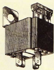
Mini Relay Make and Break, 12 volt, 15 amps, fitted with fuse.
